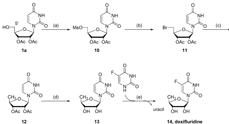
Scheme 4. Chemo-enzymatic synthesis of doxifluridine ( 14 ); experimental conditions: a) MeSO 2 Cl, pyridine, room temp. and 0 °C (yield 91%); b) Br − N + Bu 4 , DMF, 130 °C (yield 60%); c) (Bu) 3 SnH, AIBN, toluene, room temp. (yield 65%); d) MeOH/NaOMe, room temp. (yield 92%); e) immobilized uridine phosphorylase from Bacillus subtilis (UP), [21] KH 2 PO 4 buffer (pH 7.5, 10 mM), room temp. (conv.: 38%, not optimized).
