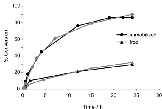
Figure 1. Enzymatic hydrolysis of peracetylated uridine, ( 1 , black) and arabinosyluracil ( 2 , gray) catalyzed by free CRL (triangle) and by immobilized CRL (circle).
