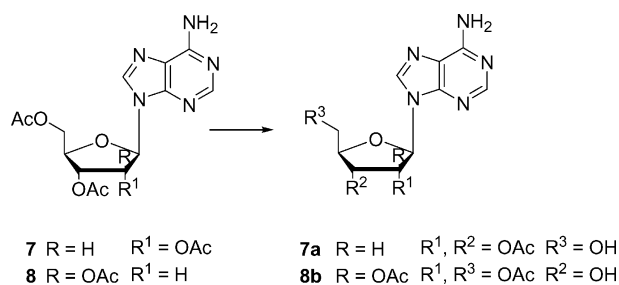
Scheme 2. Enzymatic hydrolysis of peracetylated nucleosides 7–8 ; experimental conditions: immobilized lipase, CH 3 CN (10%) in KH 2 PO 4 buffer (pH 7, 25 mM), room temp.
