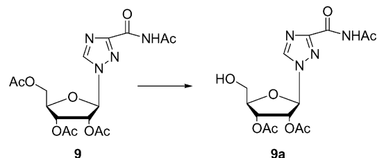
Scheme 3. Enzymatic hydrolysis of peracetylated ribavirin ( 9 ); experimental conditions: immobilized lipase, CH 3 CN (10%) in KH 2 PO 4 buffer (pH 7, 25 mM), room temp.
