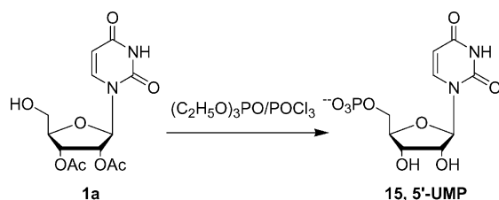
Scheme 5. Chemo-enzymatic synthesis of 5'-UMP ( 15 ).
