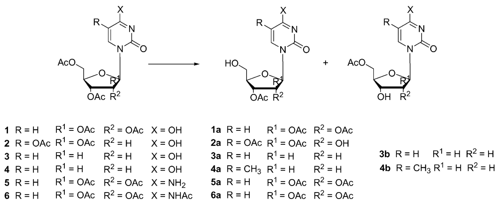
Scheme 1. Enzymatic hydrolysis of peracetylated nucleosides 1–6 ; experimental conditions: immobilized lipase, CH 3 CN (10%) in KH 2 PO 4 buffer (pH 7, 25 mM), room temp.
